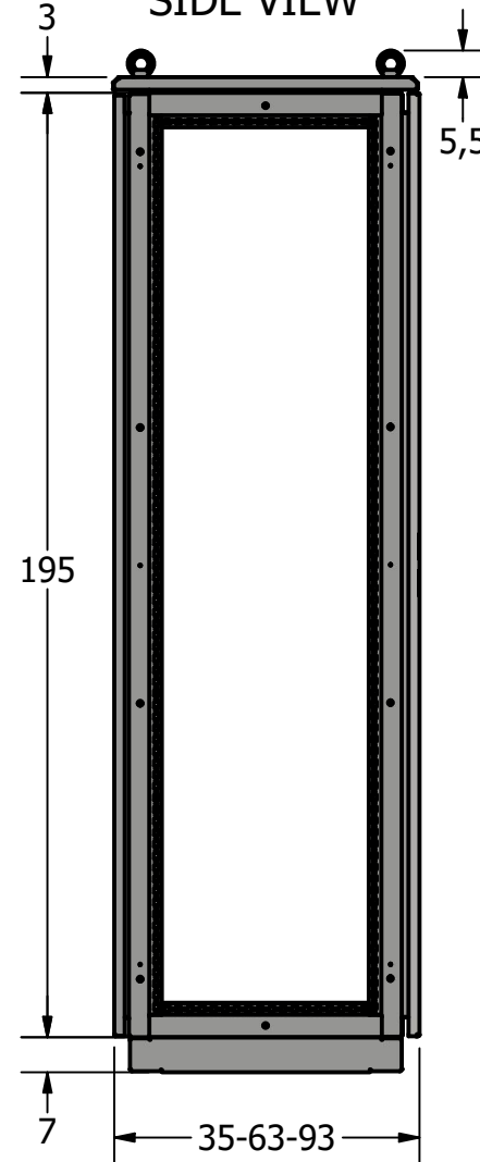
SIDE VIEW
